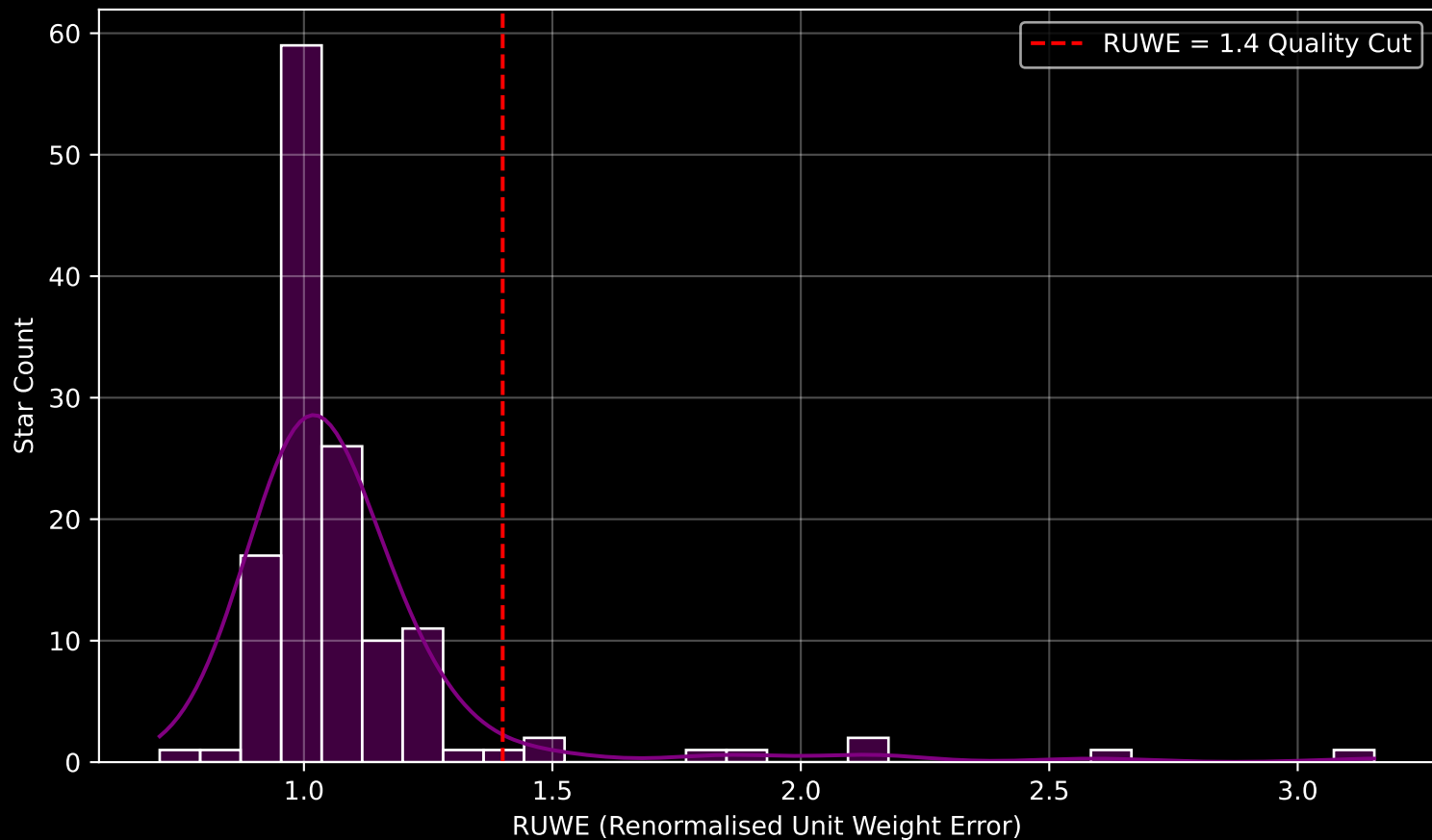
GAPOGEE DR17 Field [005+03-O] RUWE Distribution (n= 135)
