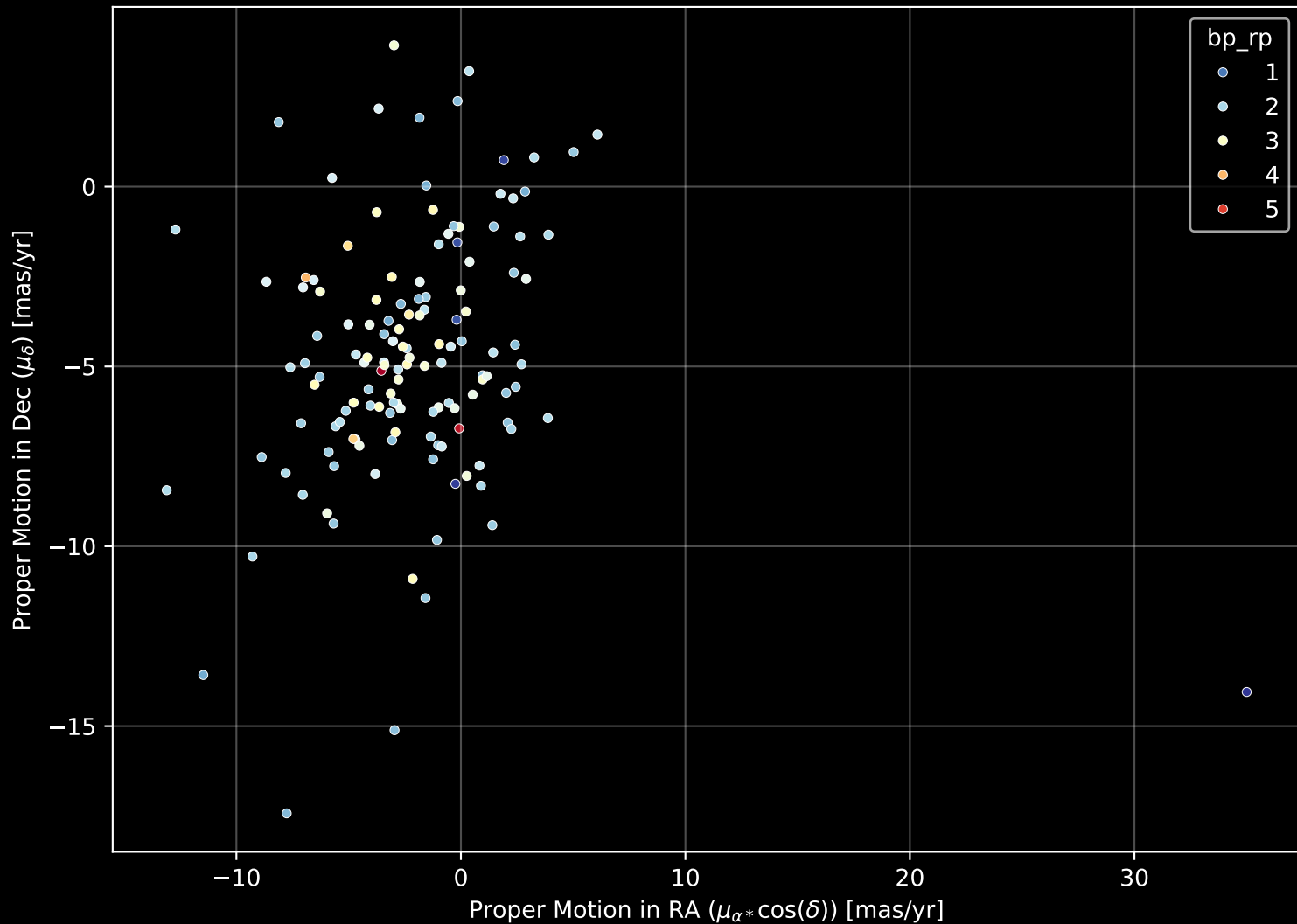
APOGEE DR17 Field: [005+03-O] Proper Motion Diagram (n= 136)
