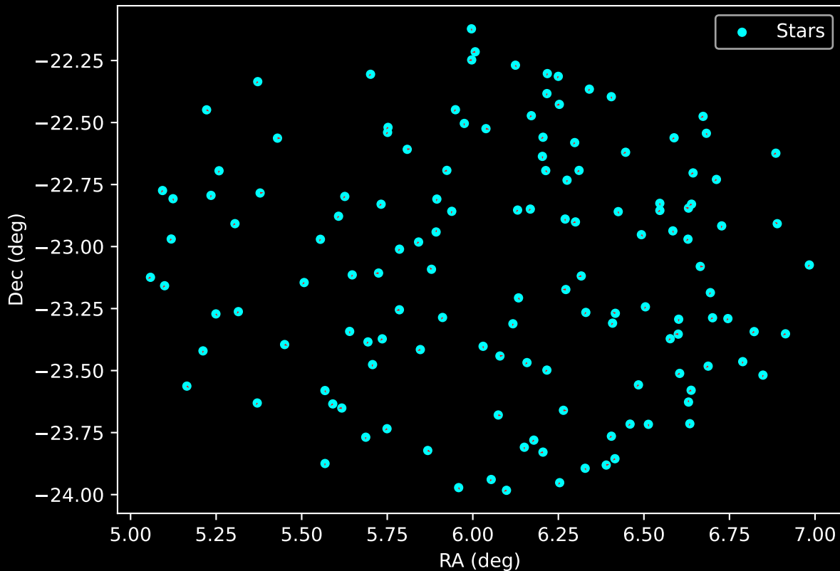
APOGEE DR17 Field: [005+03-O] Proper Motion Vectors for Gaia Star Field (n= 136)
