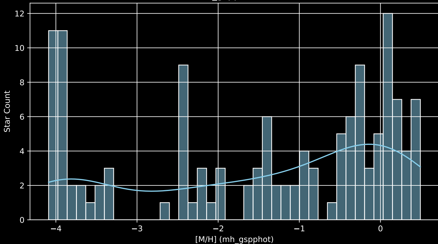
APOGEE DR17 Field: [005+03-O [M/H] (mh_gspphot) (n= 133)
