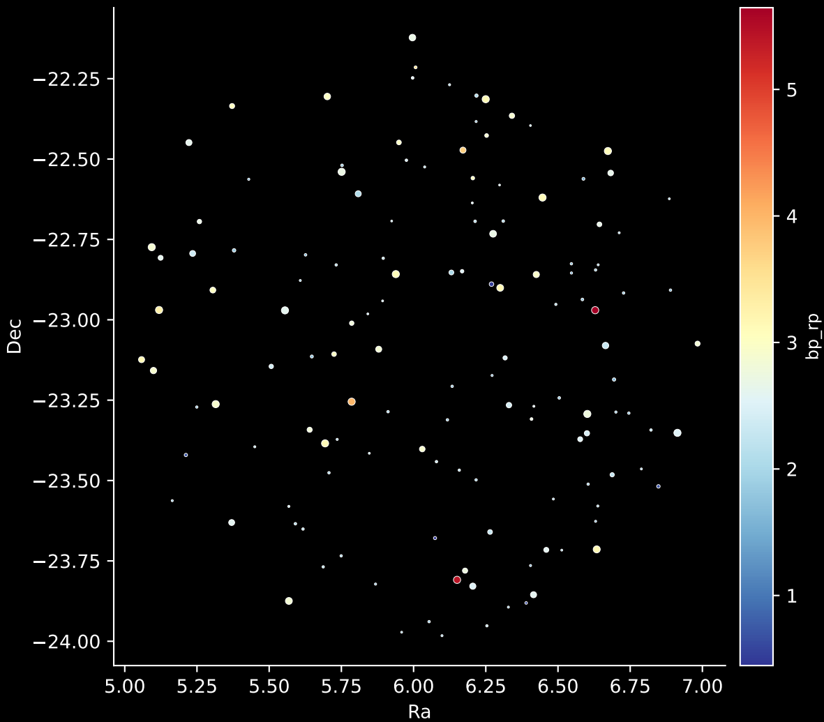
APOGEE DR17 Field: [005+03-O] Stars: 136
