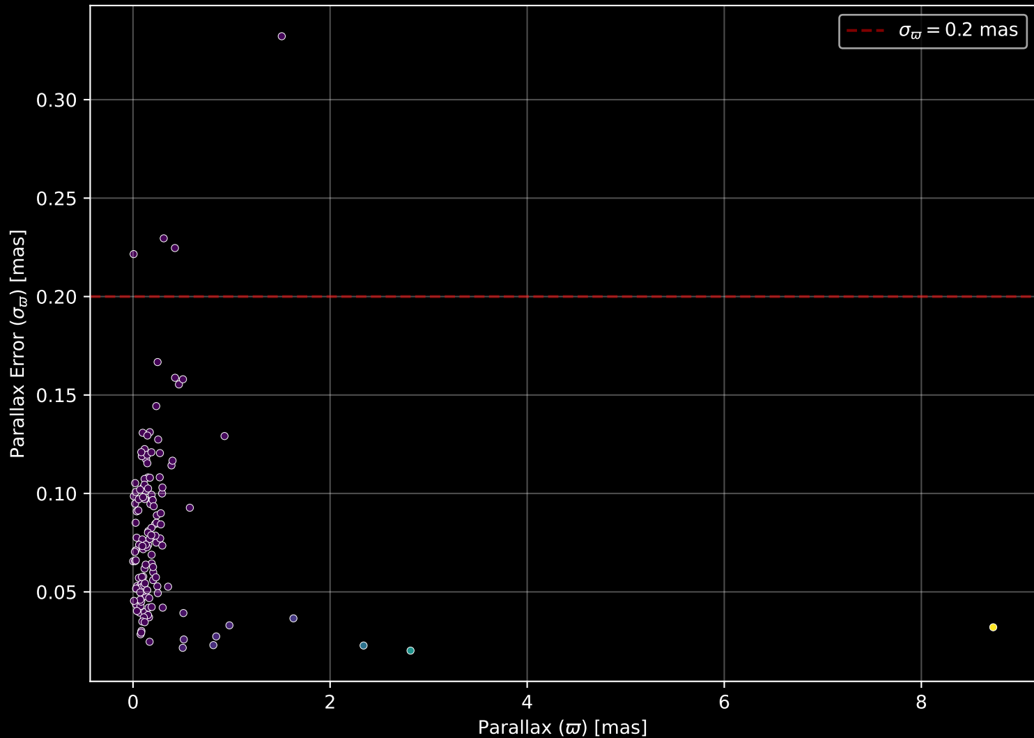
APOGEE DR17 Field: [005+03-O] Parallax Quality (n= 136)
